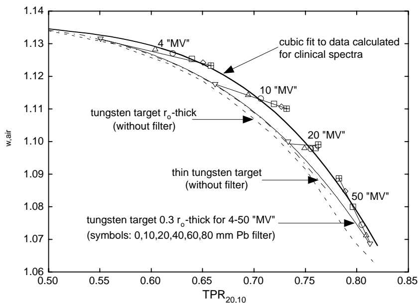
Fig. C.2. Calculated water/air stopping-power ratios for various target and filter combinations as a function of the quality of the photon beam TPR_{20,10} . Data for tungsten targets without filter are represented by the dashed-dotted line (thin target), the dashed line (thickness equal to the electron csda range in tungsten) and the thin solid line (thickness equal to one third of the electron csda range in tungsten). The symbols correspond to the r_0/3 -thick target spectra for several “MV” (for clarity a line joins the symbols for each energy) after a filtration with different thicknesses of lead (inverted triangles, no filter; normal triangles, 10 mm; circles, 20 mm; squares, 40 mm; trapezoids, 60 mm; crossed squares, 80 mm). The thick solid line is the cubic fit to data calculated for clinical beams shown in Fig. C.1. Adapted from references [53, 84].
